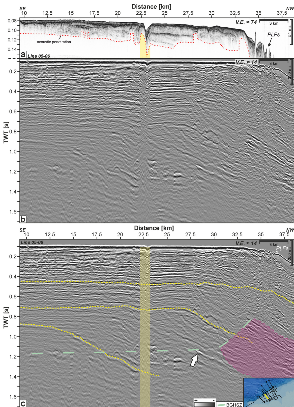
Figure 9. Co-located sub-bottom profiler data (a) and seismic section ARA05C-06 without interpretation (b) and with interpretation (c). In (a), the red dotted line shows the maximum acoustic penetration, and a yellow zone displays the same position as the yellow zone in (c). In (c), the yellow zone illustrates disturbed reflections, and the purple zone illustrates enhanced amplitudes. The yellow dotted lines show the sedimentary architecture. The light green-colored dashed line indicates the base of the gas hydrate stability zone (light green). The white arrow points at a typical bright spot. PLFs, pingo-like features.
