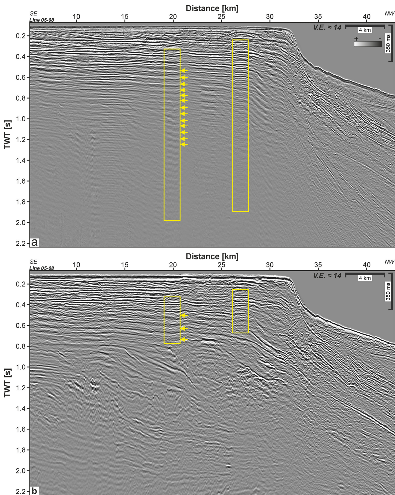
Figure 3. (a) Comparison of a conventional brute stack and (b) the corresponding final processing result of line ARA05C-08. Conventional brute stack processing: a bandpass filter, top mute, spherical divergence correction, and normal-moveout correction. A constant P-wave velocity for water of 1,500 m/s was used for the latter two. Yellow arrows point at multiples and the boxes at trains of reverberations.
